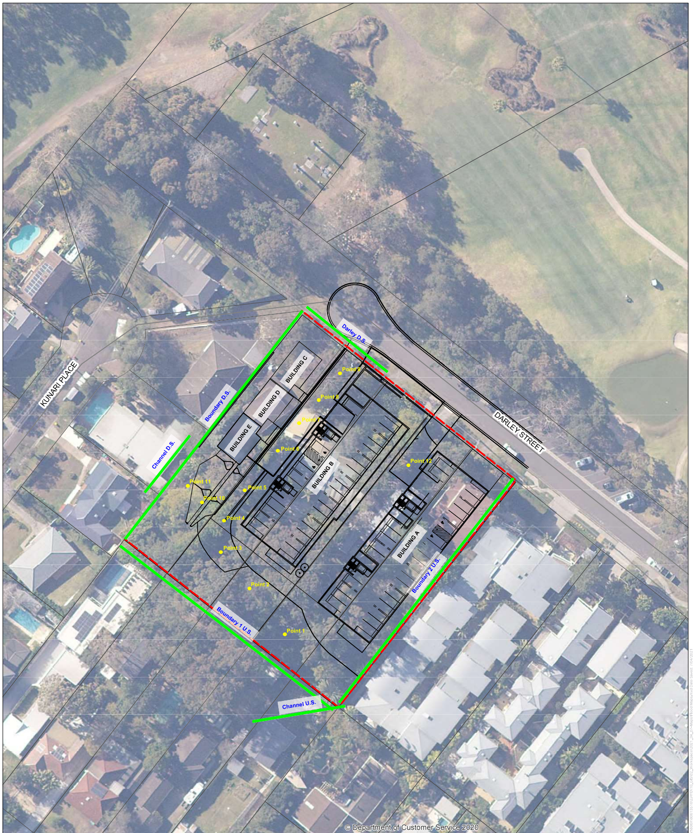
FIGURE 1: SITE LAYOUT
