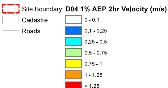
FIGURE 4: FLOOD VELOCITY (1% AEP 2 HR, DESIGN D04)
