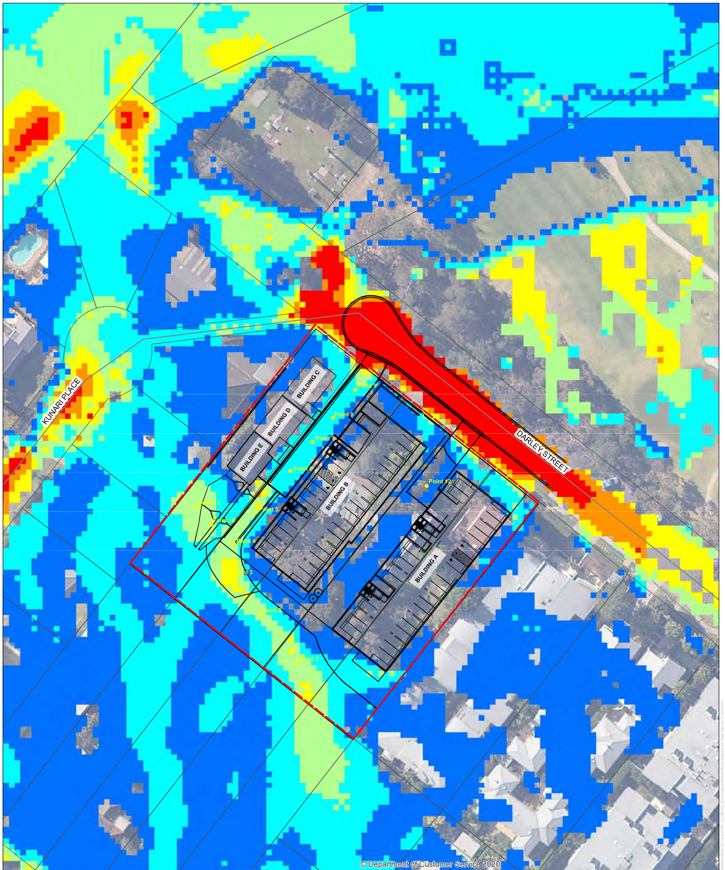
FIGURE 5: FLOOD VELOCITY (PMF 15 MIN, DESIGN D04)
