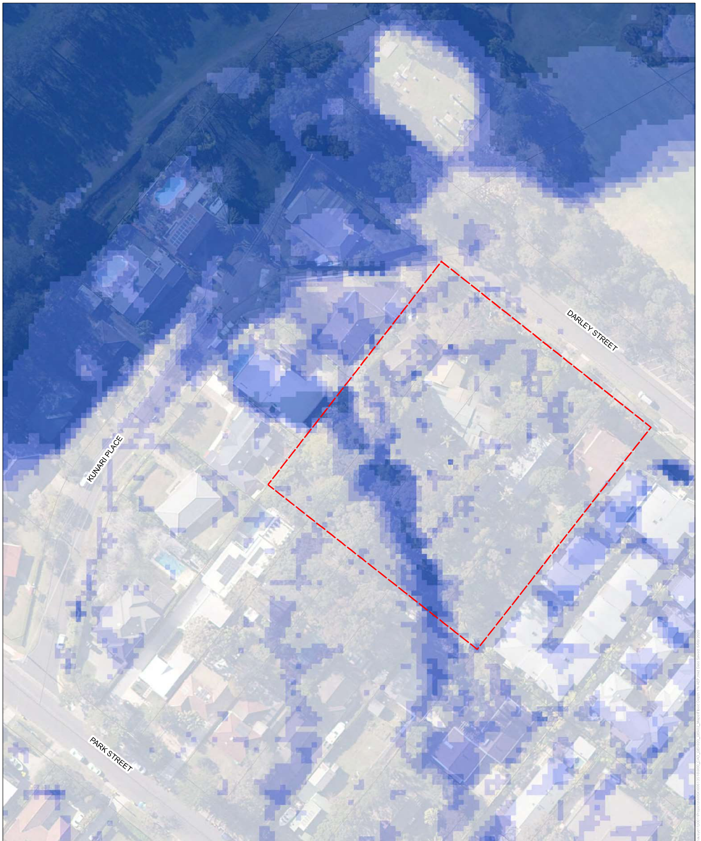
FIGURE 4: PEAK FLOOD DEPTH (PMF, 15MIN)
