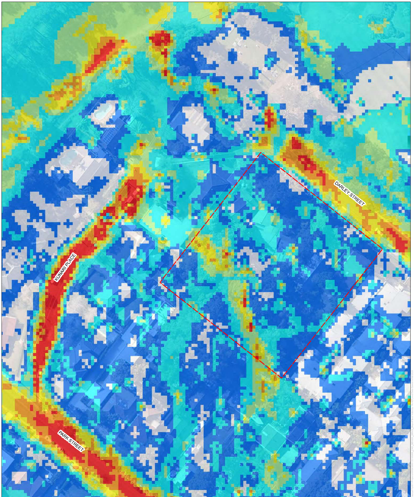
FIGURE 7: PEAK FLOOD VELOCITY (PMF, 15MIN)
