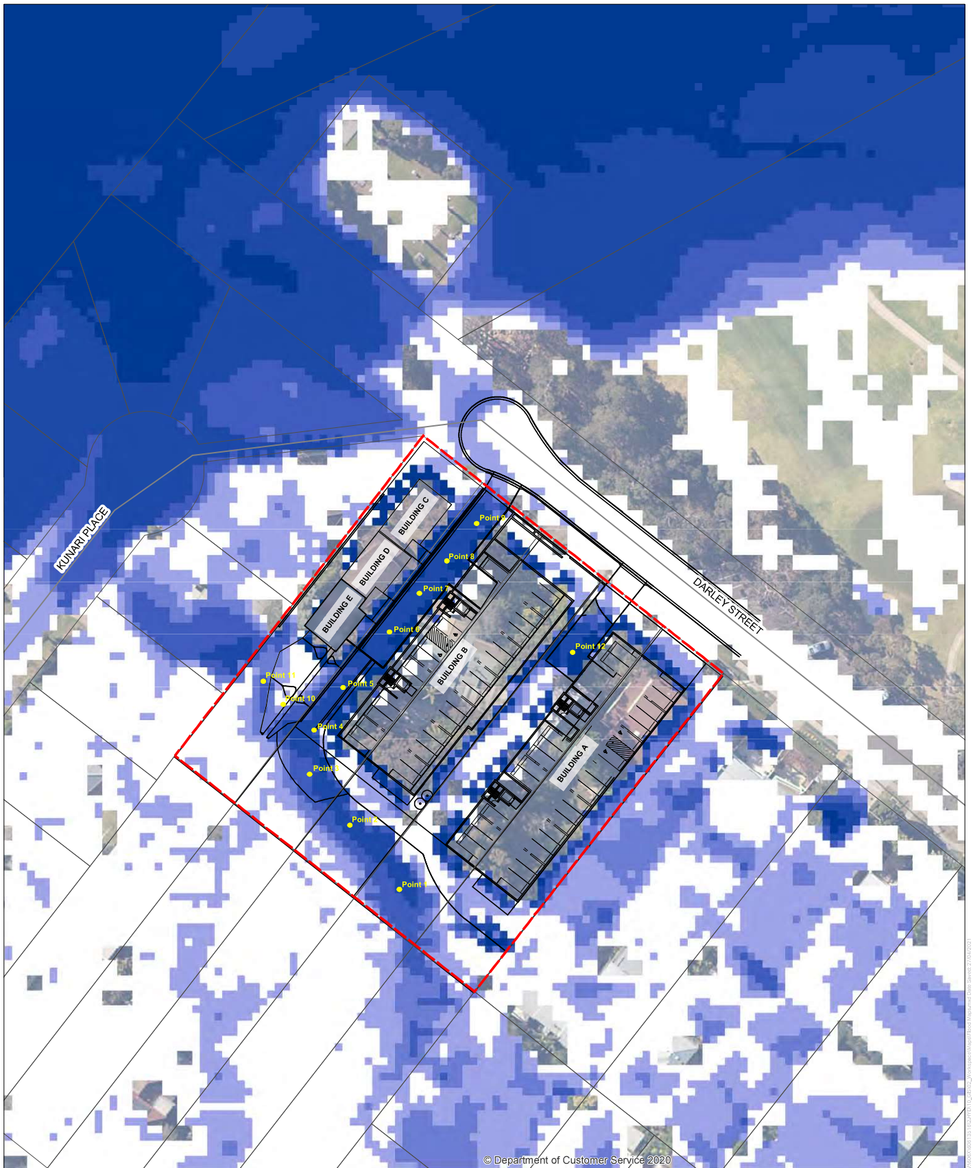
FIGURE 3: FLOOD DEPTH (PMF 15 MIN, DESIGN D04)
