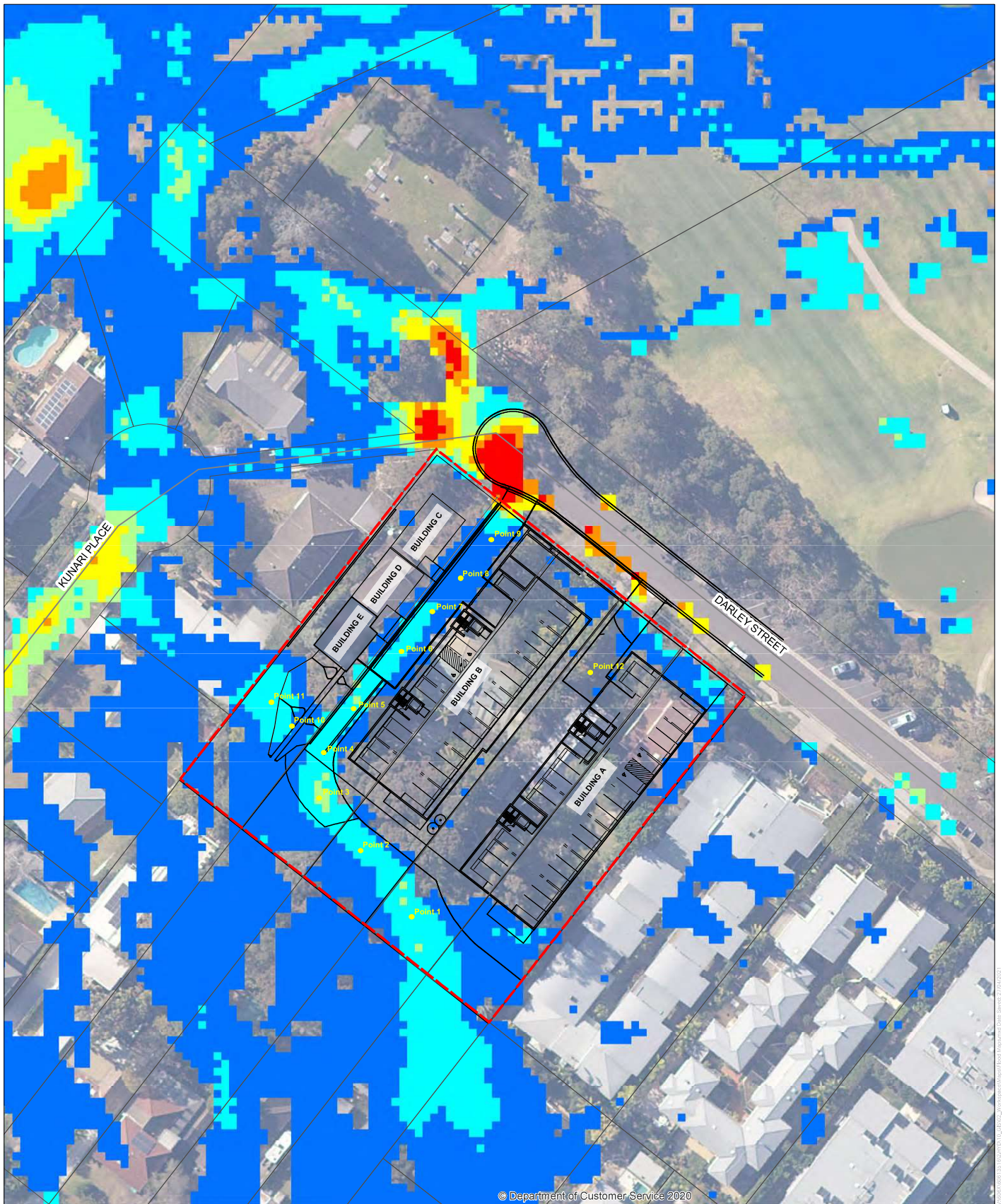
FIGURE 4: FLOOD VELOCITY (1% AEP 2 HR, DESIGN D04)
