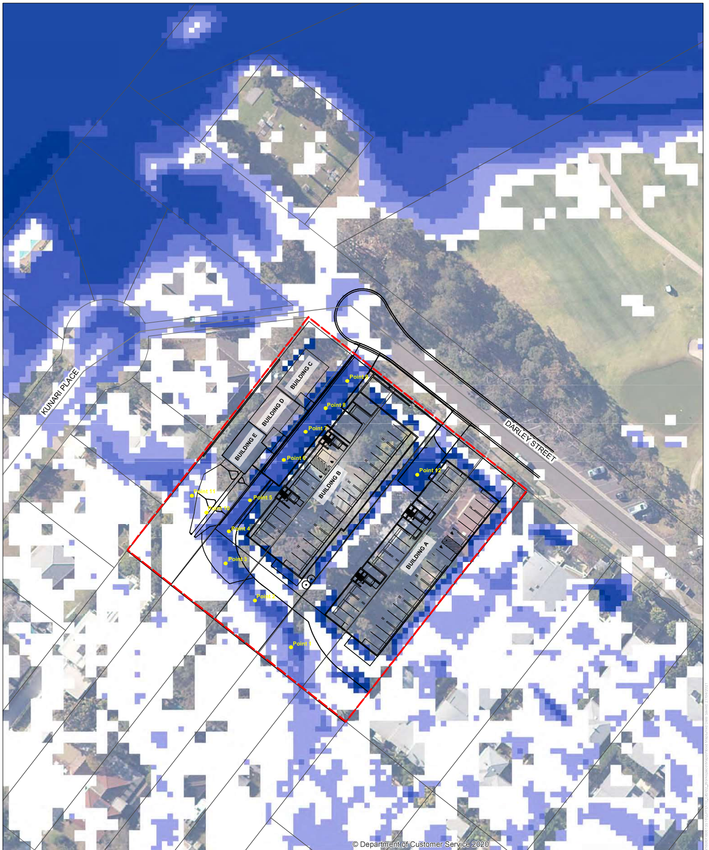
FIGURE 2: FLOOD DEPTH (1% AEP 2 HR, DESIGN D04)
