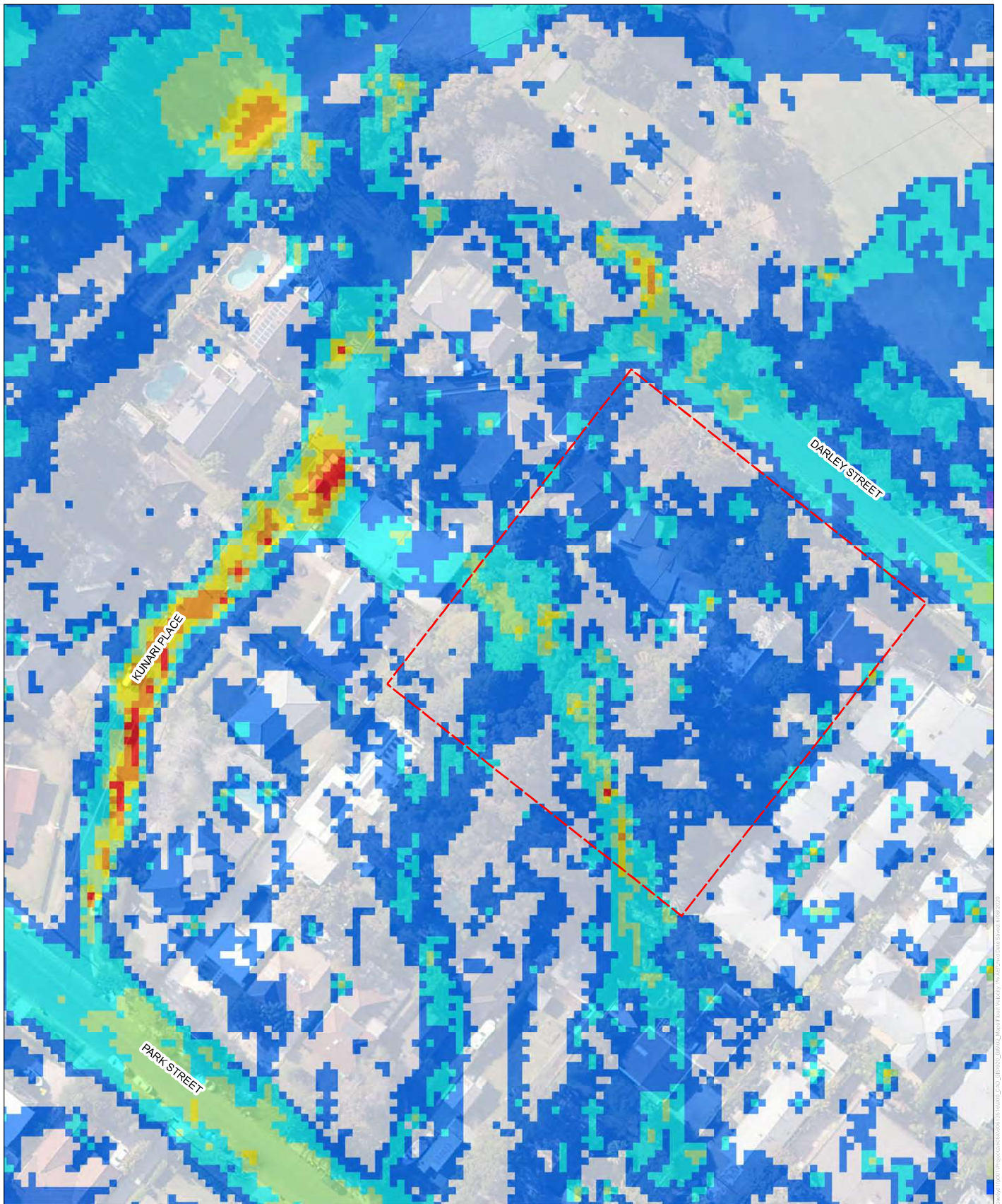
FIGURE 6: PEAK FLOOD VELOCITY (1% AEP, 2HR)
